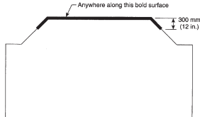
LOCATIONS PERMITTED FOR SMOKE ALARMS ON TRAY-SHAPED CEILINGS
